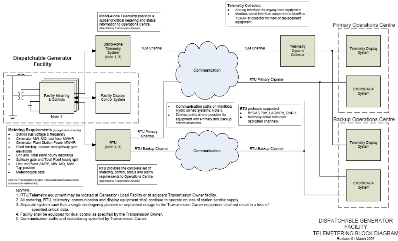
Figure 3: Manitoba Hydro Dispatchable Generator Facility Telemetry Block Diagram
