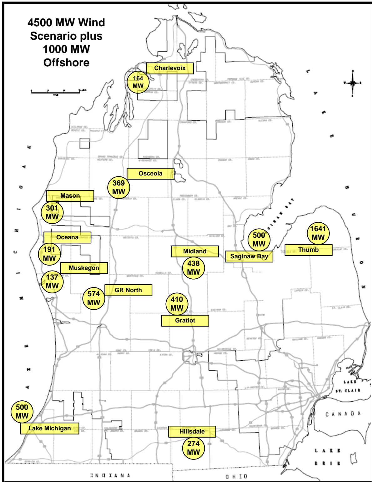
FIGURE 4.3.6—LOCATIONS FOR 4500 MW WIND SCENARIO PLUS 1000 MW OFFSHORE
