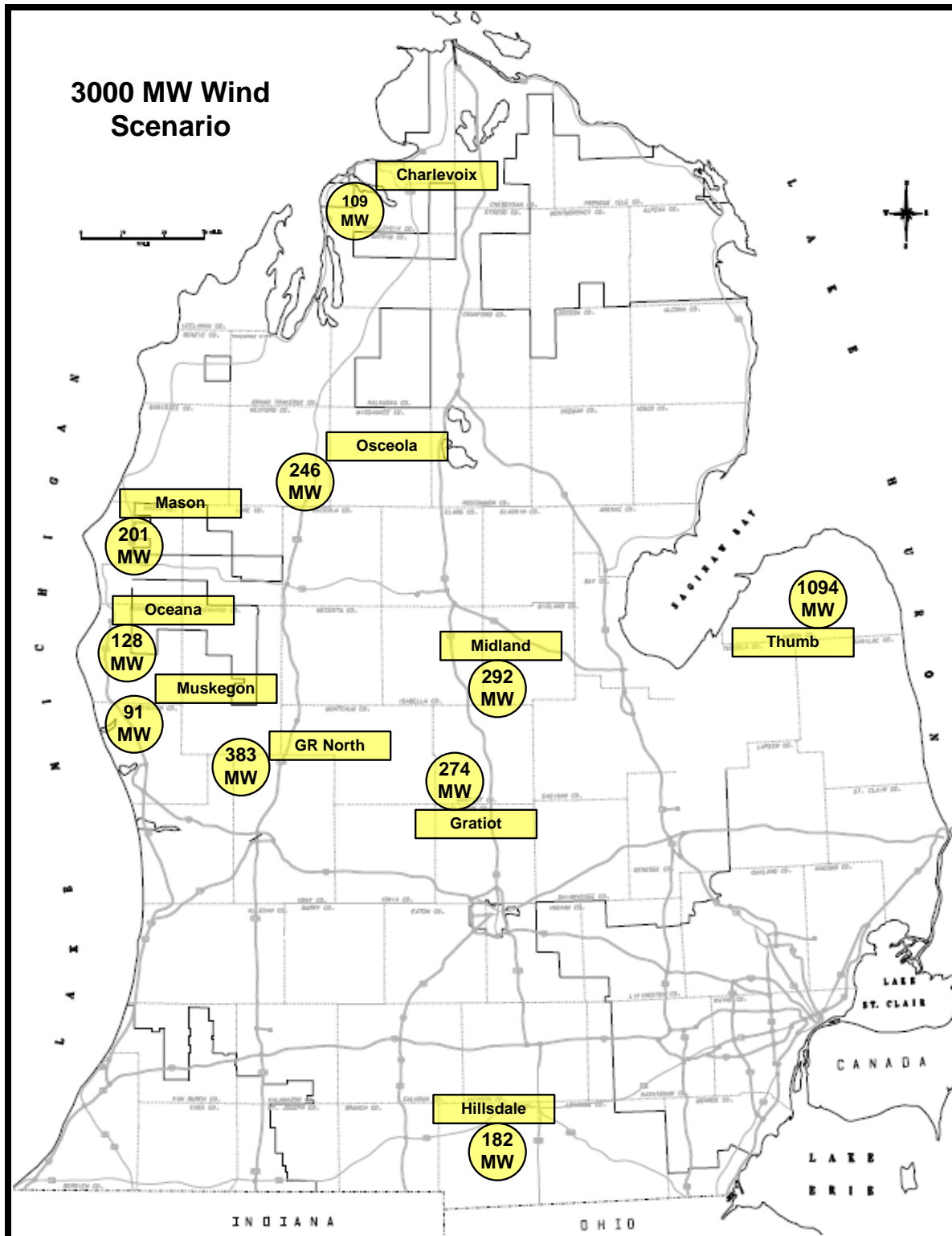
FIGURE 4.3.4 – LOCATIONS FOR 3000 MW WIND SCENARIO
