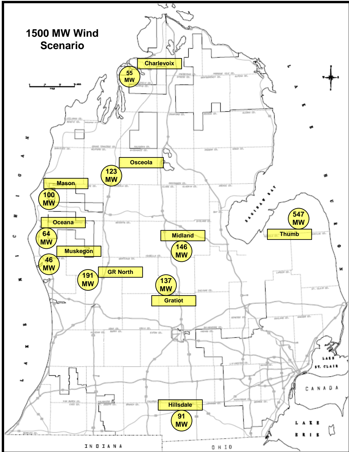
FIGURE 4.3.3 – LOCATIONS FOR 1500 MW WIND SCENARIO
