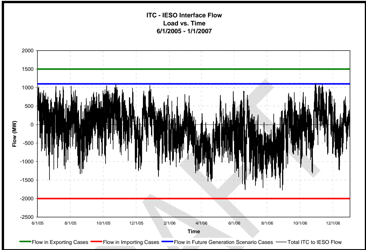
FIGURE 4.1.1 – HISTORICAL ITC – IESO INTERFACE FLOW
