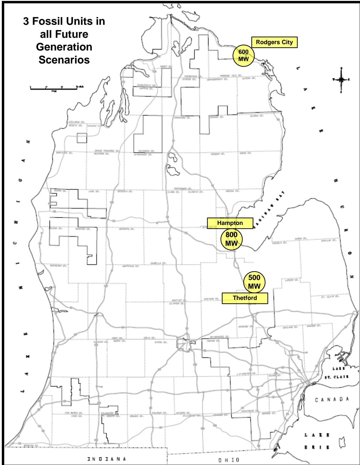
FIGURE 4.3.2 – 3 FOSSIL UNITS USED IN ALL FUTURE GENERATION SCENARIOS
