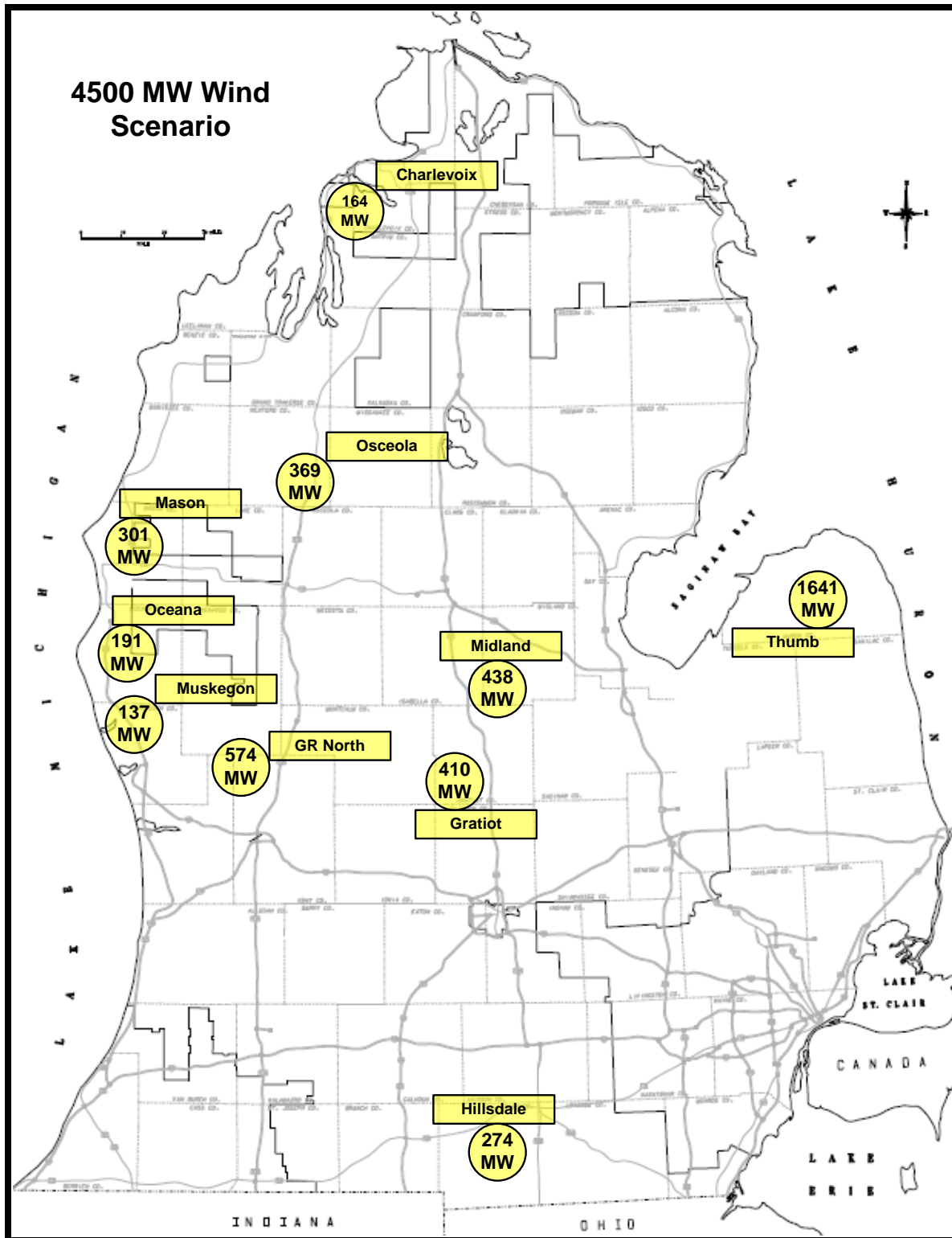
FIGURE 4.3.5 – LOCATIONS FOR 4500 MW WIND SCENARIO
